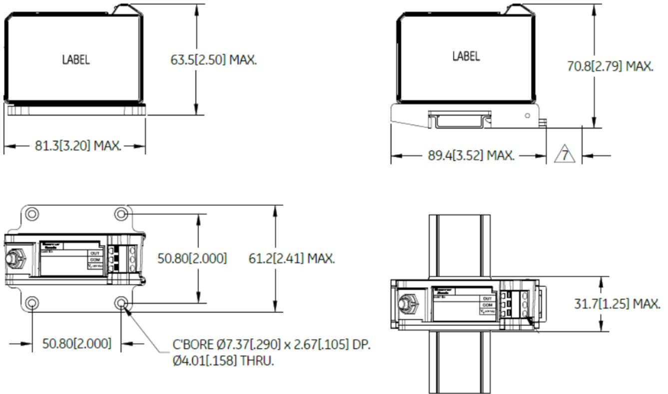
Figure 11: 330380 HTPS Proximitor Sensor (see drawing of same number)
