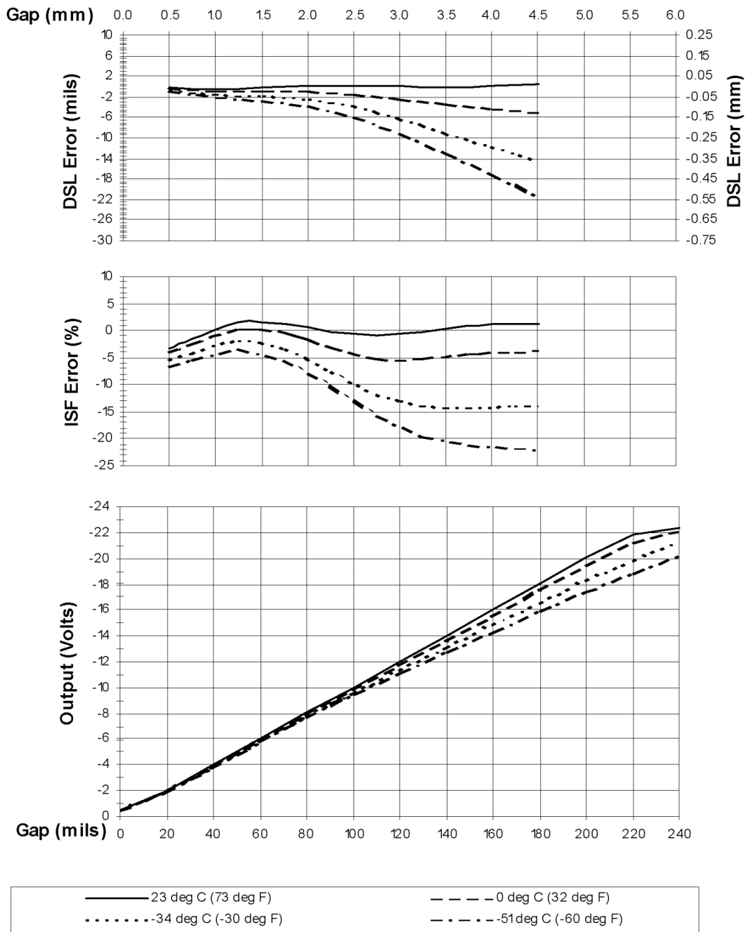
Figure 5: Typical 3300 XL HTPS Performance with Proximitor Sensor at Low Temperature
